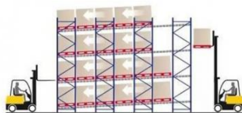
Pallet Flow Racking
