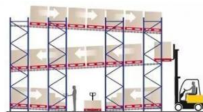
Case picking from the pallet
